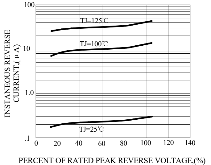
FIG.4-TYPICAL REVERSE CHARACTERISTICS
